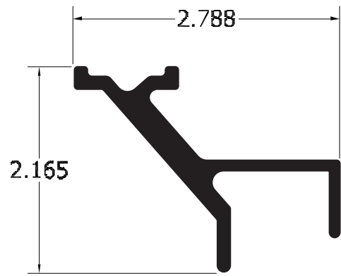
Small Frame Brace Part# 5352
